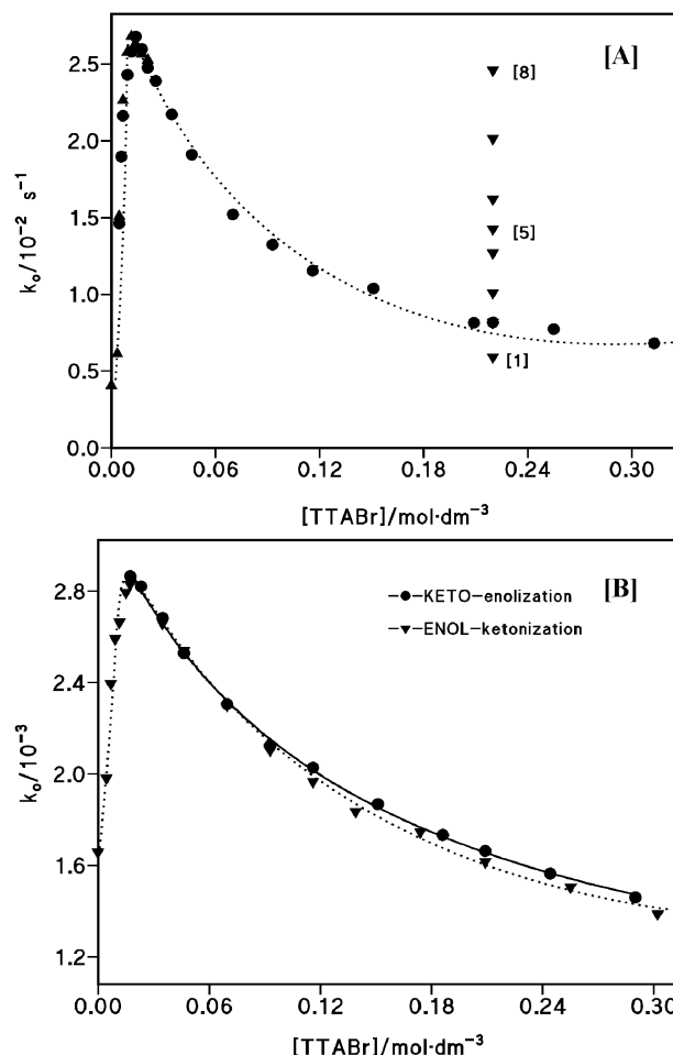
Fig. 6 Rates of keto-enol tautomerization measured in aqueous micellar solutions of TTABr for (A) 2-acetylcyclohexanone at [buffer] = 2.67 mM (acetic acid:acetate in a 1 : 1 ratio) and (B) 2-acetyl-1-tetralone at (●) [buffer] = 1.33 mM and (▼) 0.22 M of TTABr and variable buffer concentrations (e.g., [8] 6.7 mM; [5] 3.3 mM, and [1] 0.67 mM).
