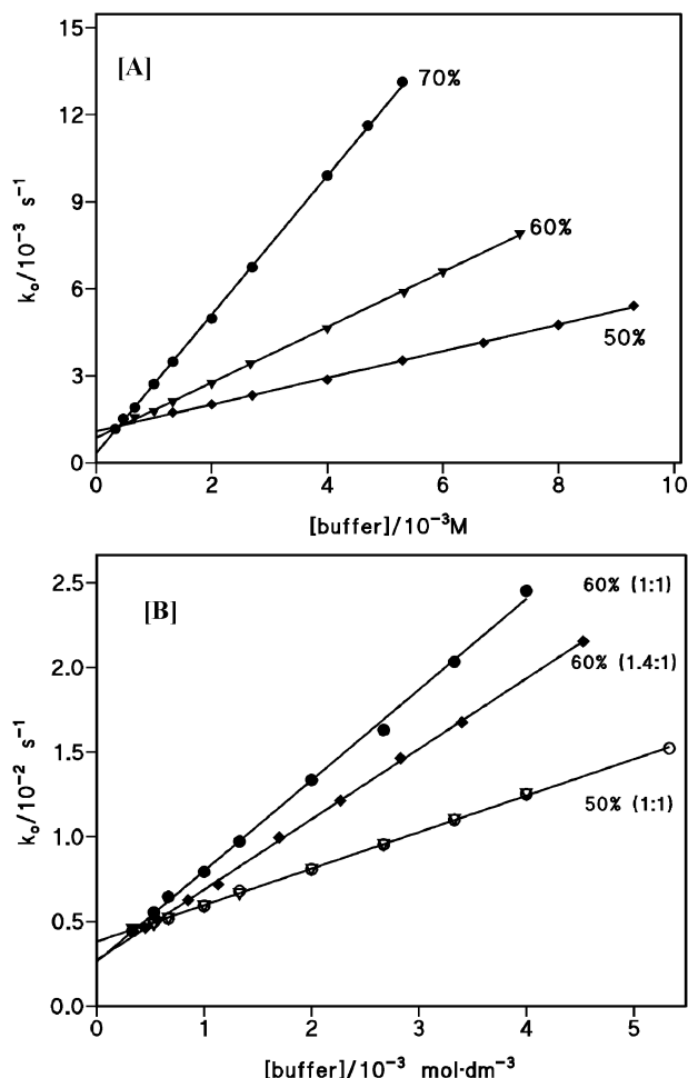
Fig. 2 Pseudo-first-order rate constants, k_o , for keto-enol tautomerization of (A) ACHE determined as a function of buffer concentration at 70%, 60% and 50% DMSO and a 1:1 ratio of AcOH:AcO - , and (B) ATLO determined at 60% and 50% DMSO, and at ratios of AcOH:AcO - equal to 1:1 and 1.4:1 for (●,◆,○) keto-enolization and (▽) enol-ketonization.
