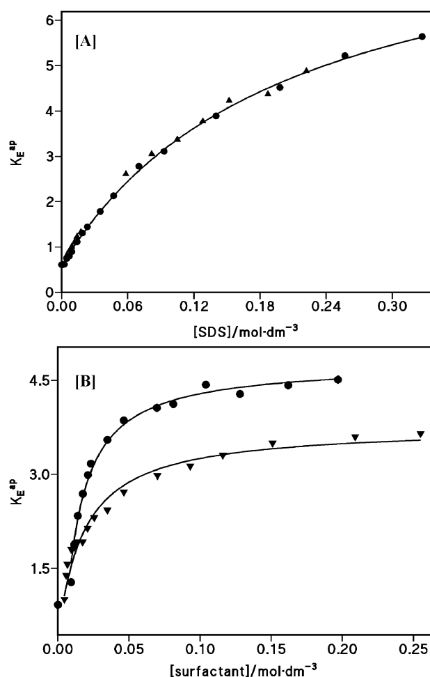
Fig. 8 Plots of K_E^{\text{ap}} against [surfactant] corresponding to (A) ACHE determined in (●) 0.030 M HCl; (▲) 0.13 M acetic acid–acetate, 1 : 1, and (B) ATLO in 1.33 mM acetic acid–acetate, 1 : 1, in (●) SDS and (▼) TTABr. The lines are fits from eqn. (6); for results, see Table 4.
